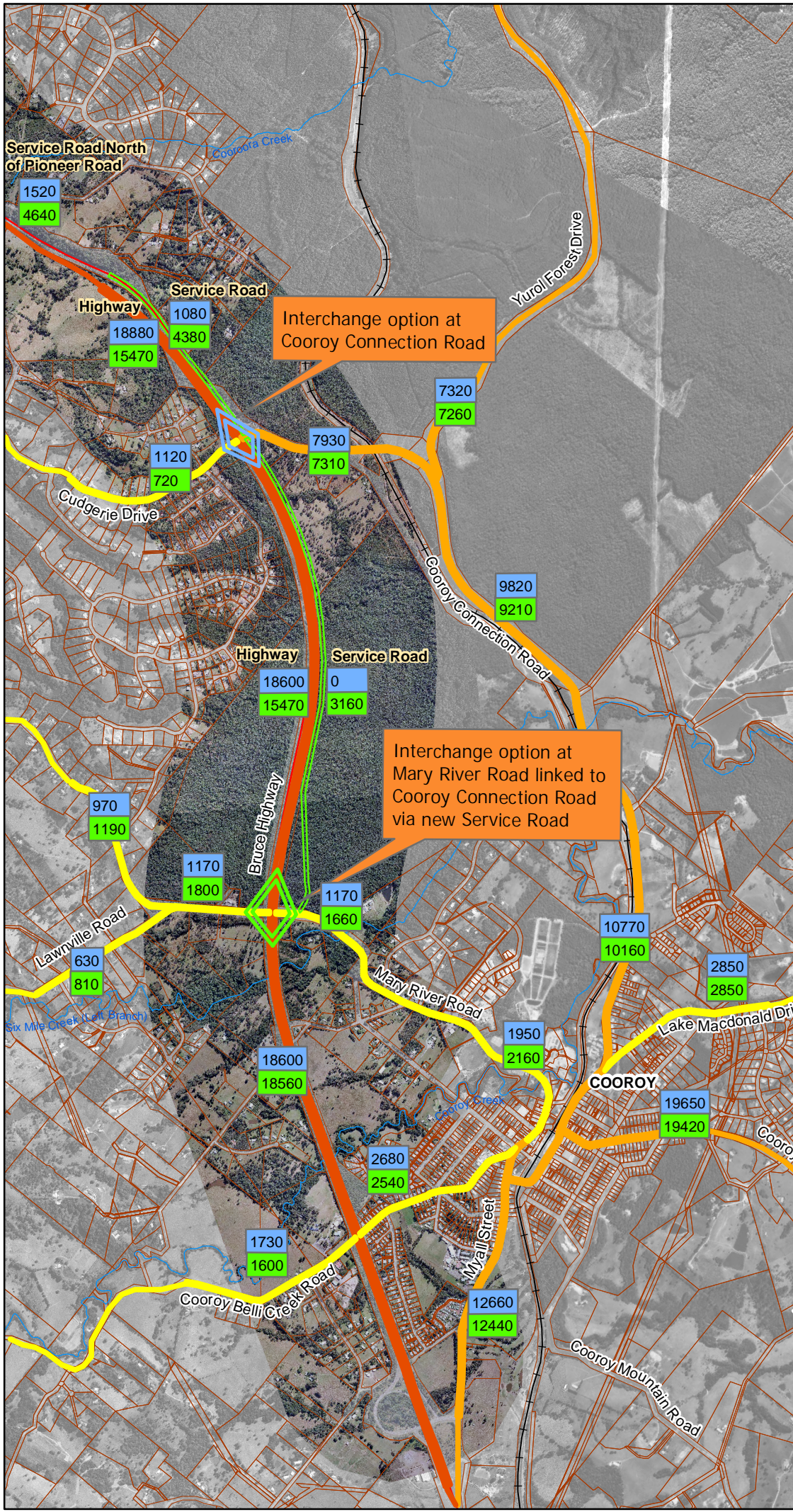
Figure 3.1b Forecast 2026 (Cooroy Region) Traffic Volumes
